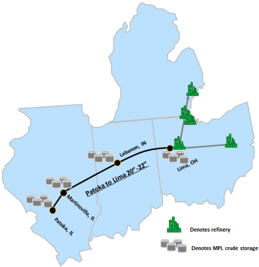
Patoka to Lima crude system overview
